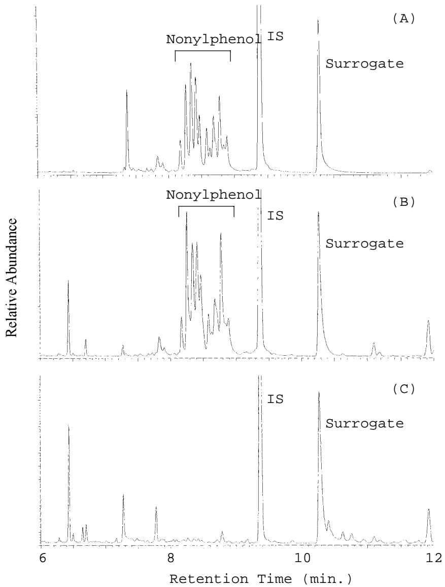
Fig.1 GC-MS chromatograms of standard solution (A), sample no.15 (B), and sample no.16 (C).
